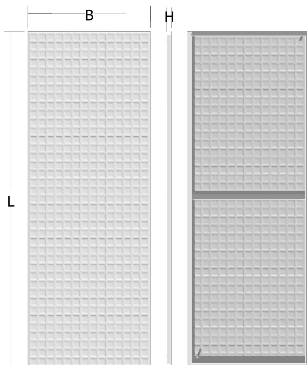
Fig. 3 – KIGO Paneel – B x L x H
